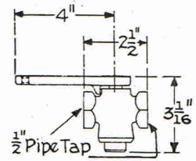
Cut Out Cock Cat. 38565 Approx. Weight 1 1/2 lb.
