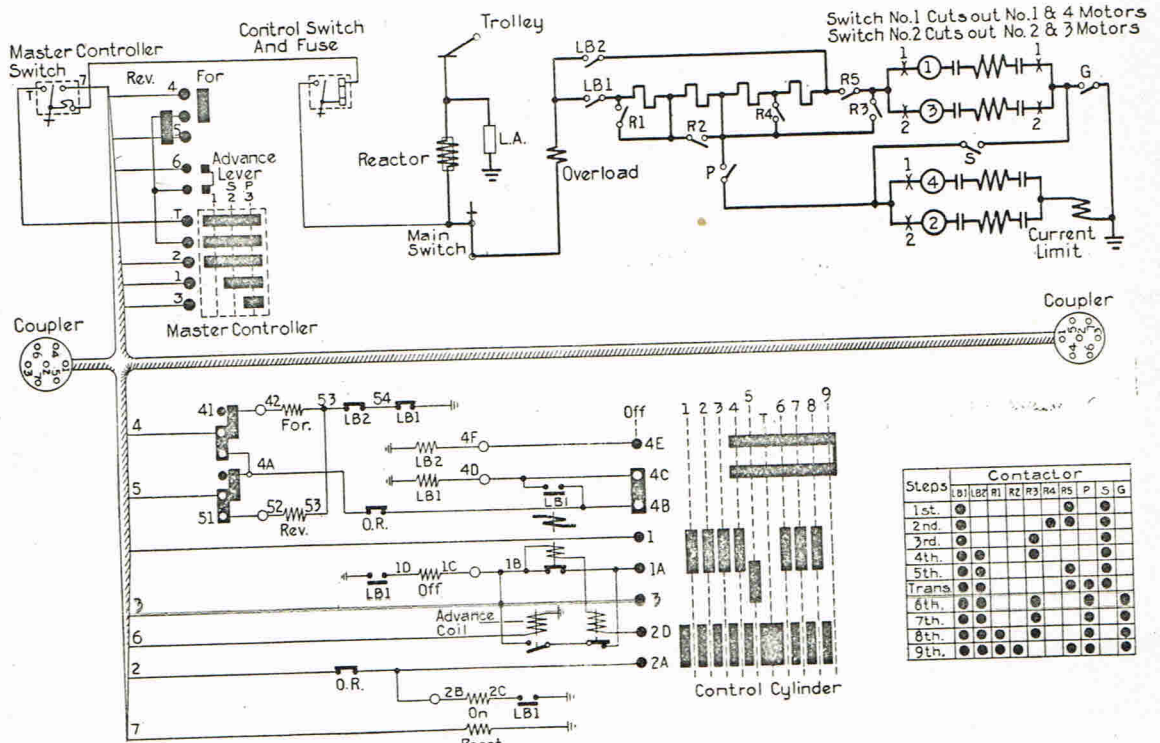
Fig. 15. Connections of PC-12 Controller and Four Motors
