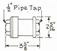
Strainer Approx. Weight 1 1/2 lb.
