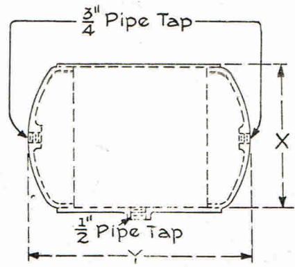
Reservoir
