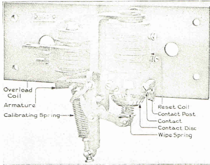
Fig. 34. Overload Relay for Types PC-5, PC-6 and PC-9 Controllers
