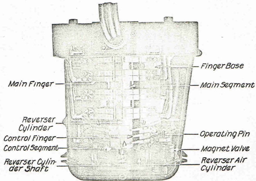
Fig. 37. Reverser for PC-10 Controller
