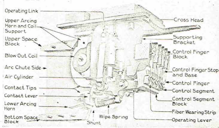
Fig. 32. Line Breaker Unit for Types PC-5, PC-6 and PC-9 Controllers
