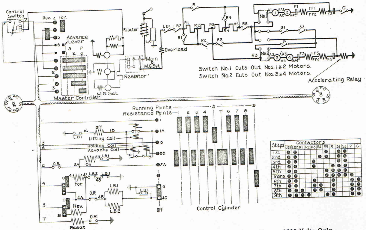
Fig. 16. Connections of PC-101 Controller and Four Motors. Operation on 1500 Volts Only
