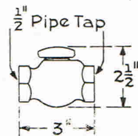
Check Valve Approx. Weight 1 1/2 lb.
