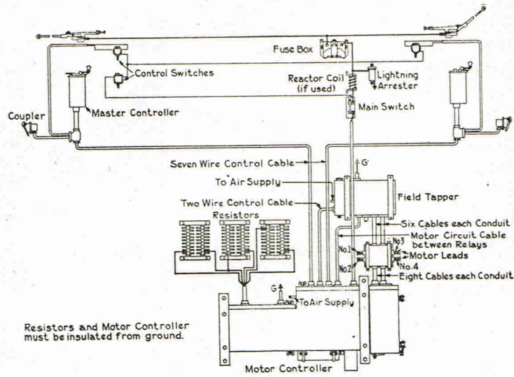
Fig. 7. Motor Controller Arrangement of Car Equipment with PC-5 Controller and Field Tapper
