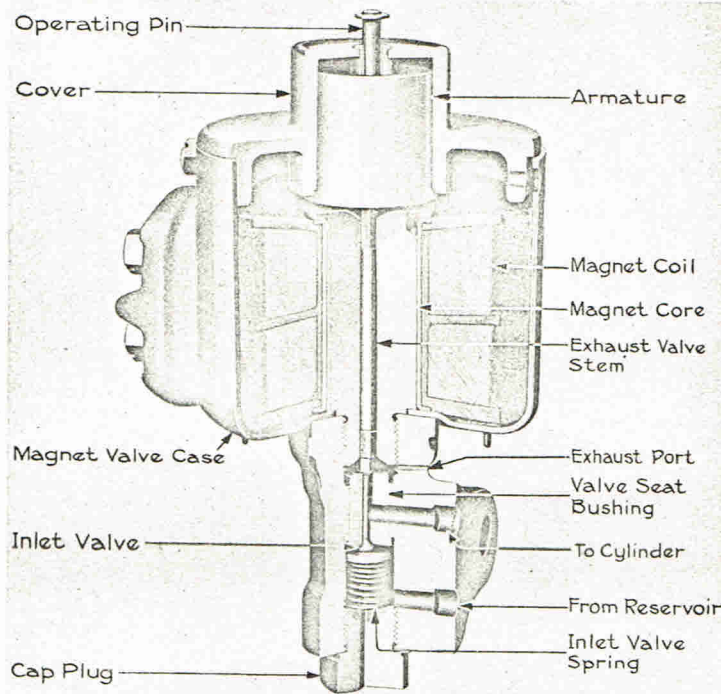
Fig. 41. Magnet Valve for Reverser, Line Breaker and "ON" Cylinder
