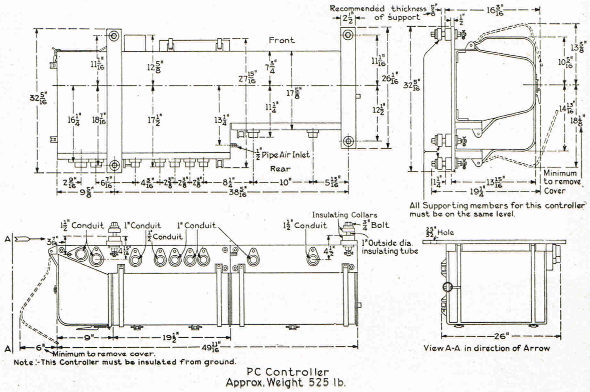
Fig. 5. Outline of Small PC Controller for Two or Four Motors, 600 Volts
