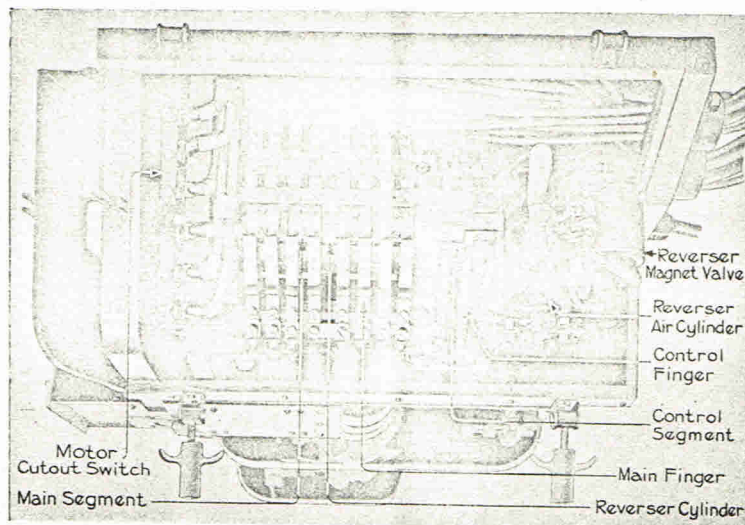
Fig. 33. PC-5 Controller (Reverser End)
