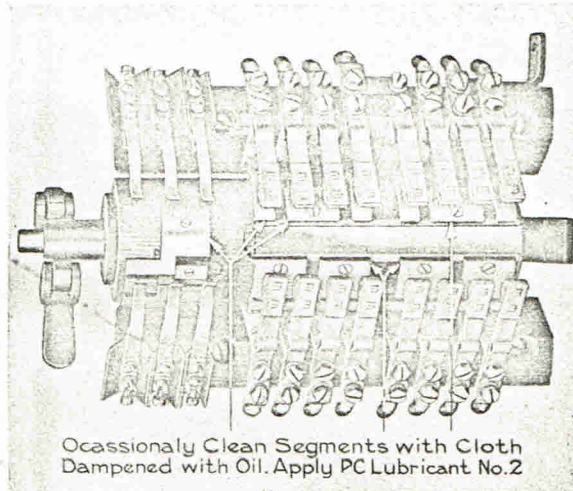
Fig. 48. Lubrication Chart of Reverser
