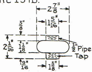
Pipe Insulation Joint Cat. 1609 Approx. Weight 1/2 lb.
