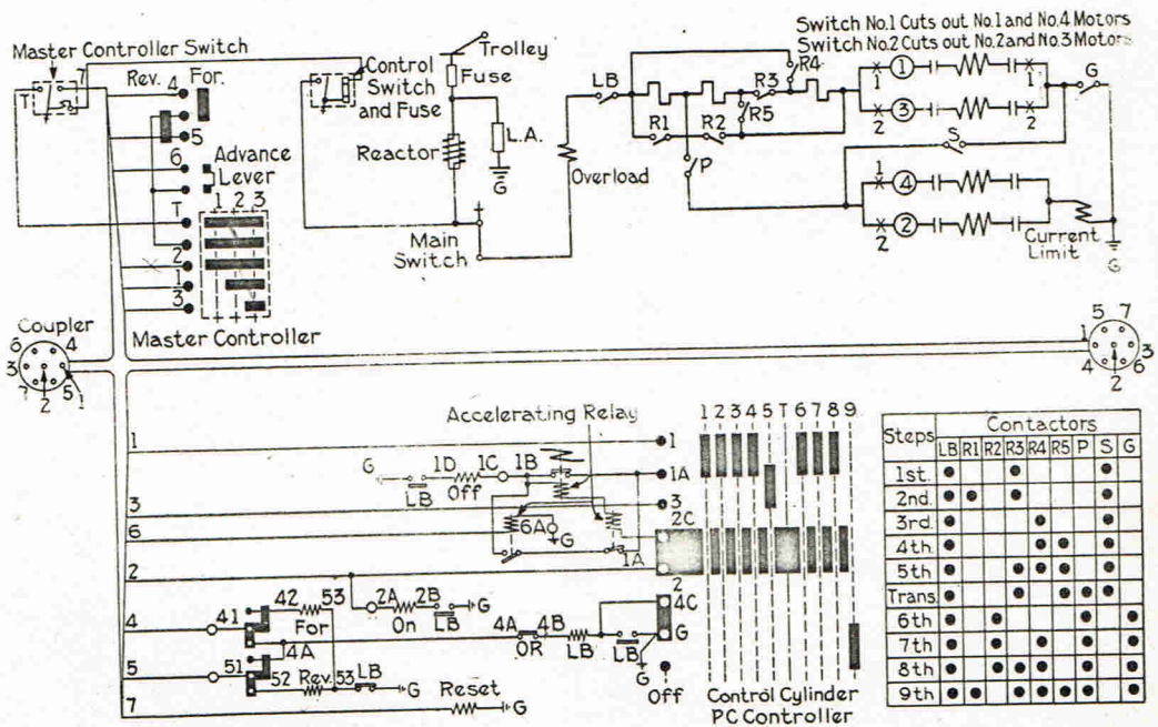
Fig. 8. Connections of PC-5 Controller and Four Motors
