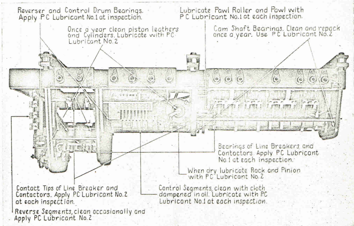
Fig. 43. Lubrication Chart for PC-10, PC-12, PC-13, PC-14, PC-101 and PC-102 Controllers
