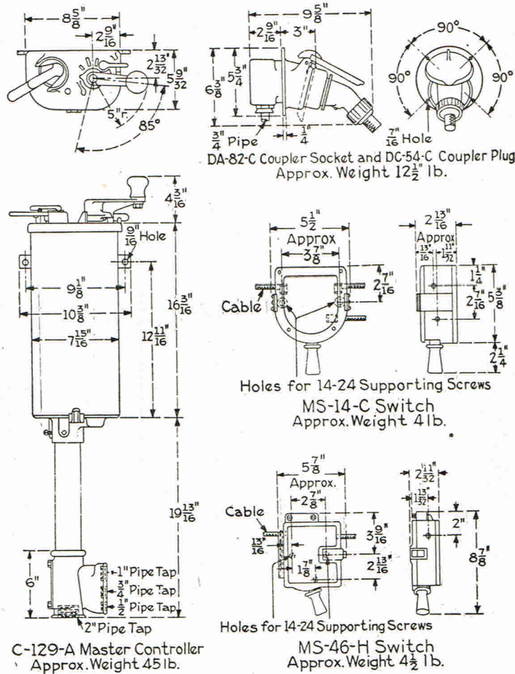
Fig. 21. Outlines of Electrical Apparatus Used with 600-volt PC Controllers
