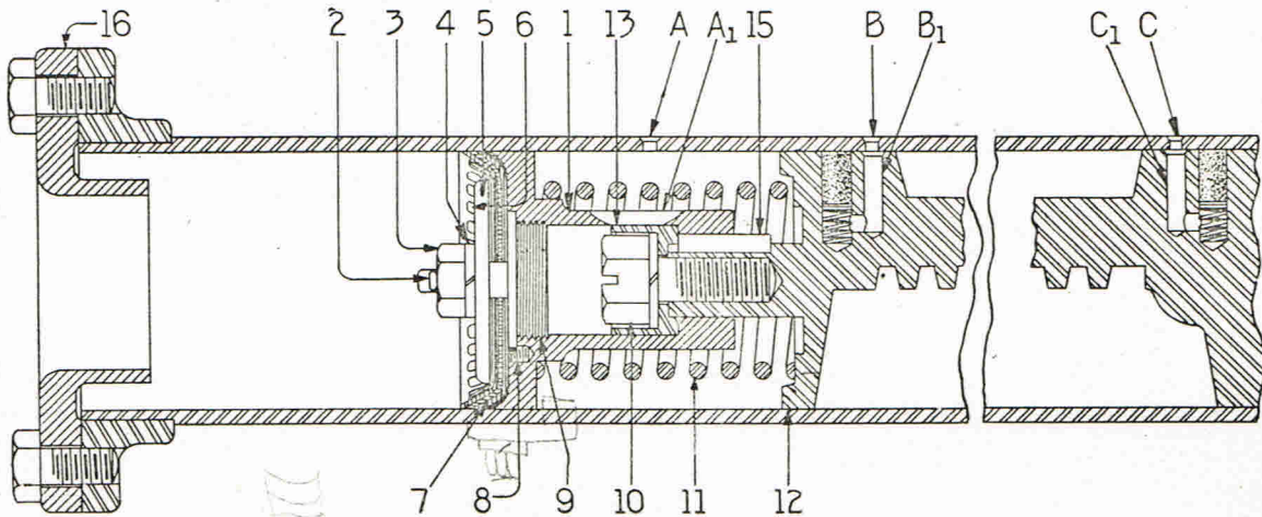
Fig. 29. Section Through Main Cylinder Showing Piston for Types PC-10, PC-12 and PC-101 Controllers
