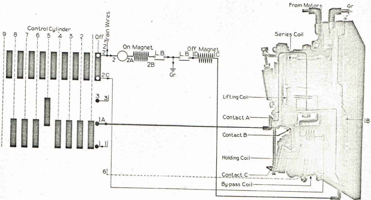
Fig. 40. Type DB-808 Relay (Control Connections)
