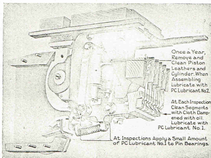
Fig. 47. Lubrication Chart of Line Breaker
